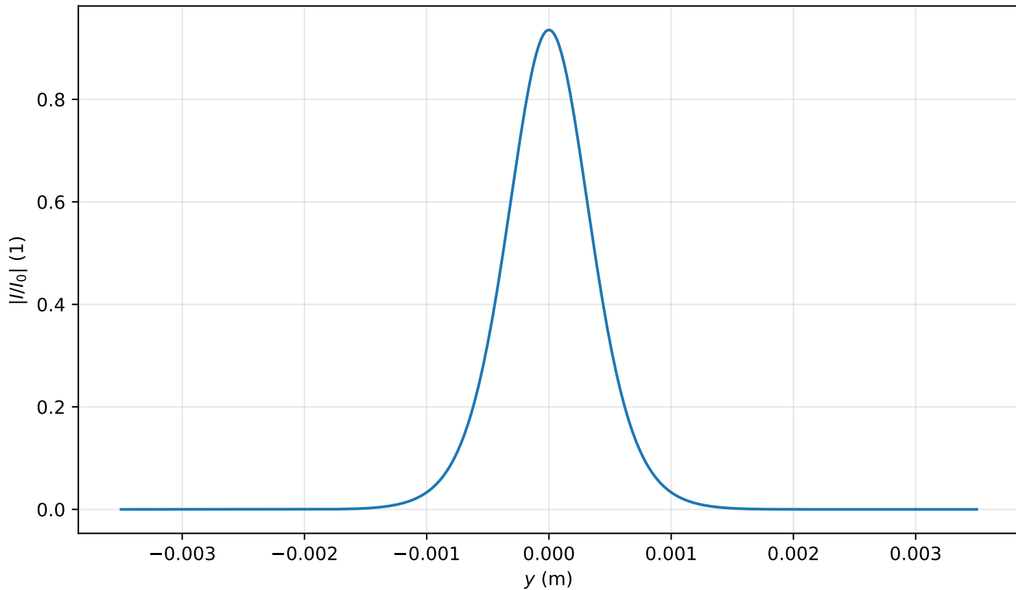
Intensity profile I(x=0, y, z=1.592)/I_0 , P_{in}=0.5P_{cr} , artificial time
